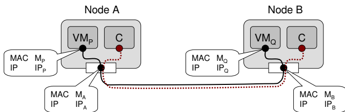
Figure 2. Challenges for the use of the path-coupled signaling model in a virtual network environment
